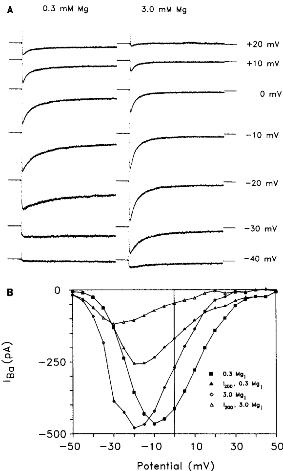
FIGURE 7. Effects of [Mg^{2+}]_i on kinetics of inactivation of I_{Ba} at different potentials. I_{Ba} was evoked by 800-ms duration pulses from -80 mV to the potential indicated. Traces were leak-subtracted. External [Mg^{2+}] was 0 mM. (A) Sample leak-subtracted current traces obtained at the voltages shown from the same cell perfused internally with either 0.3 mM [Mg^{2+}]_i or 3.0 mM [Mg^{2+}]_i . (B) Current-voltage relationships for I_{Ba} in the same cell. (Solid squares) Leak-subtracted peak I_{Ba} amplitude with 0.3 mM [Mg^{2+}]_i . (Solid triangles) Amplitude of I_{Ba} at 200 ms after onset of pulse with 0.3 mM [Mg^{2+}]_i . (Open diamonds) Leak-subtracted peak I_{Ba} amplitude with 3 mM [Mg^{2+}]_i . (Open triangles) Amplitude of I_{Ba} at 200 ms with 3 mM [Mg^{2+}]_i . (C) Time constants of fits of I_{Ba} . Inactivation of Ba^{2+} currents were fit to the sum of two exponentials plus an offset [I_t = A * \exp(-t/\tau_1) + B * \exp(-t/\tau_2) + C] . The amplitudes (A, B, and C) were normalized
