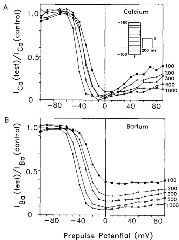
FIGURE 3. Time course of inactivation of I_{\text{Ca}} and I_{\text{Ba}} . ( A ) I_{\text{Ca}} inactivation. Internal solution contained 1.0 mM [\text{Mg}^{2+}] . External solution contained 1.8 mM \text{CaCl}_2 , 1.8 mM \text{MgCl}_2 . A two-pulse inactivation protocol consisted of a prepulse to the voltage indicated on the x-axis of duration 100-ms ( squares ), 200 ms ( pluses ), 300 ms ( diamonds ), 500 ms ( crosses ), or 1,000 ms ( inverted triangles ) followed after a 3-ms interval by a test pulse to 0 mV of 200 ms duration. The amplitude of the response to the test pulse preceded by a prepulse was plotted as a fraction of the amplitude of the response to the test pulse in the absence of a prepulse. ( B ) I_{\text{Ba}} inactivation from the same cell as in A . The solutions and conditions were the same as in A except that 2 mM \text{BaCl}_2 replaced 1.8 mM \text{CaCl}_2 in the external solution.
